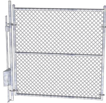
6' 1829 mm T-Pin with Keeper Pin: 45032-WWF-CP
